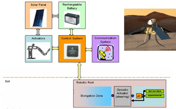
Figure 4: Elements of the plantoid involved in operating the technical roots.
