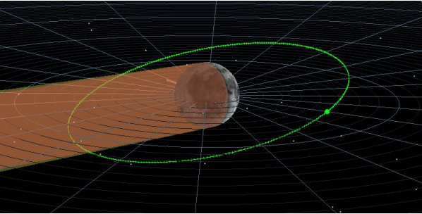
FIG. 1: Umbra cone in the proximities of the Moon
