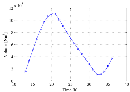
Figure 8. Single station storage without SPS
