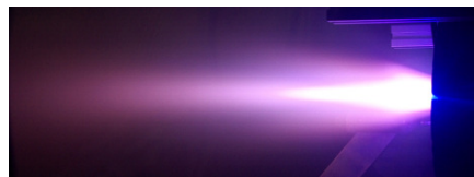
Figure 1: Plume of the AF-MPD ZT1 thruster in steady-state operation with 5.4 kW (Argon)
