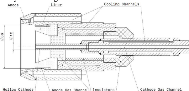
Figure 4: Sectional view of new 100 kW AF-MPD SX3 thruster (redesigned AF-MPD ZT2) [2]
