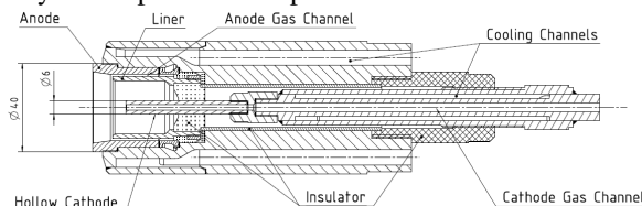
Figure 3: Sectional view of new AF-MPD SX1 thruster (Improved AF-MPD ZT1)
