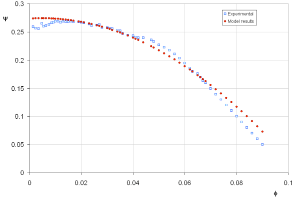
Figure 5. Comparison between the experimental noncavitating performance of the MK1 inducer (blue) and the prediction of the analytical model (red).
