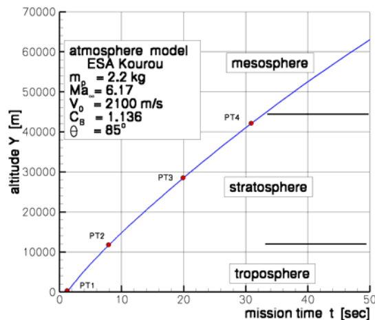
Figure 6 First 50 seconds of flight for the proposed projectile configuration
