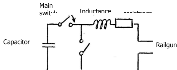
Figure 13 Scheme of the electric circuit used to feed the railgun
