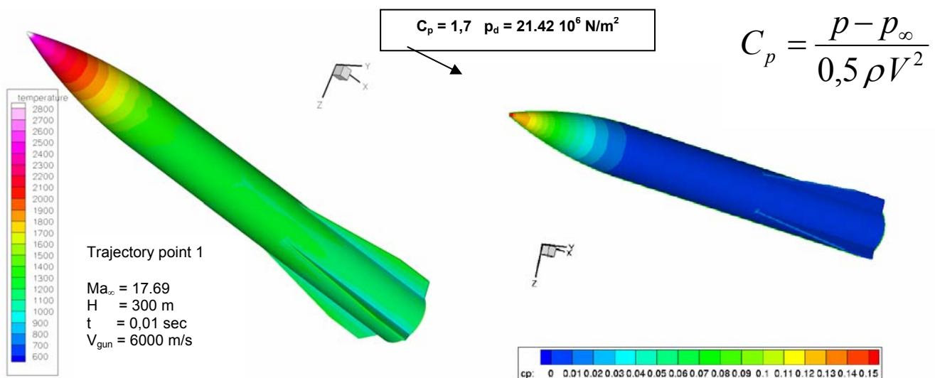
Figure 25 Propelled projectile surface temperature distribution
