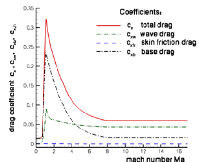
Figure 4 Drag coefficient changes with Mach number
